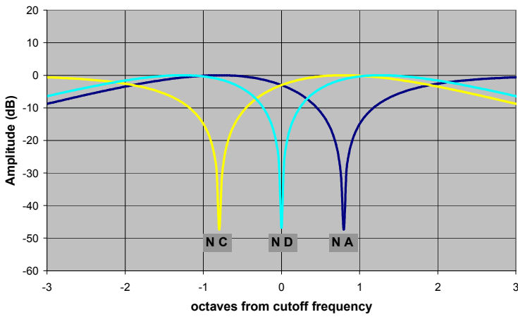
Notch Frequency Responses -- Zero Resonance
