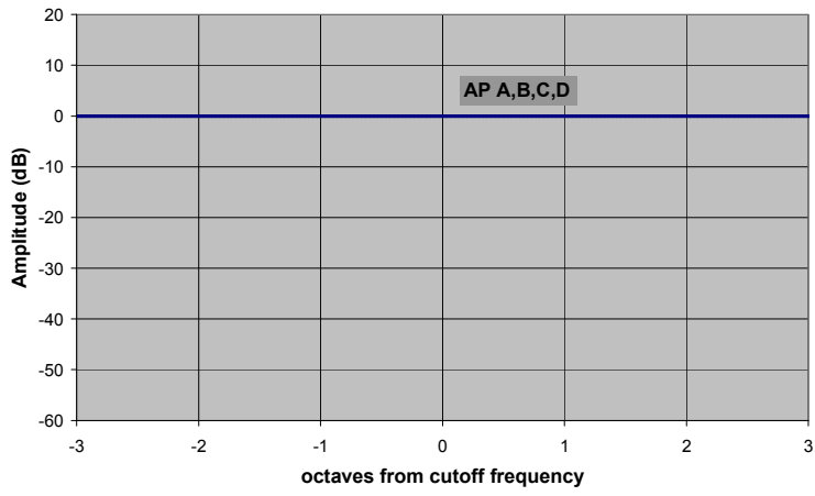
All Pass Frequency Responses -- Zero Resonance
