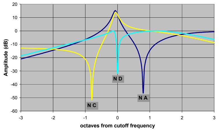
Notch Frequency Responses -- 90% Resonance
