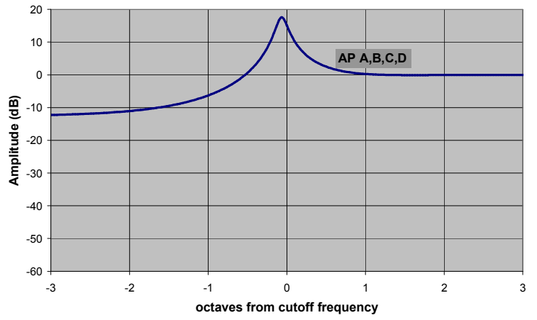
All Pass Frequency Responses -- 90% Resonance
